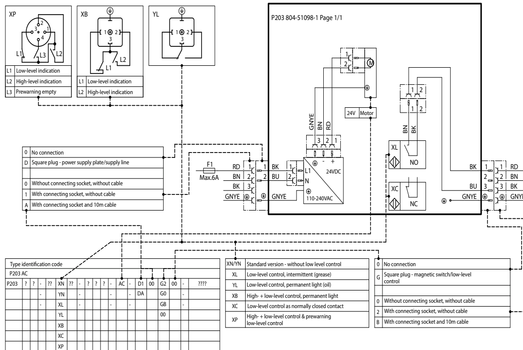
Connection diagram P203 V AC without control PCB Fig. 32
