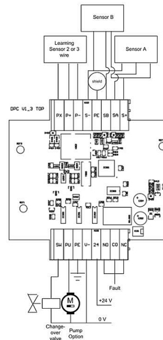
Circuit diagram 4
